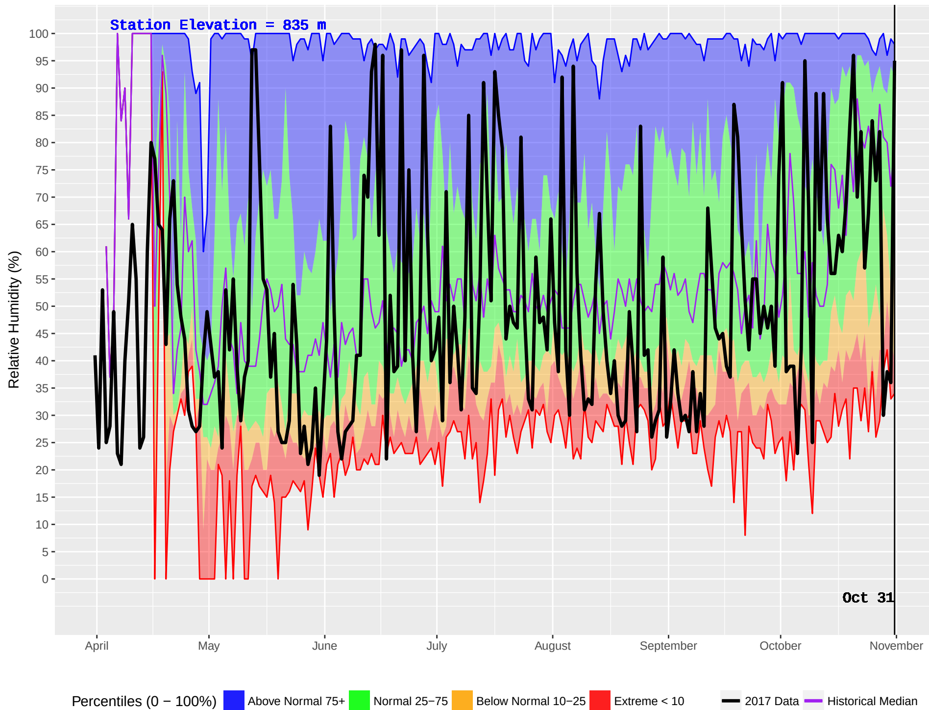
SILVER (120) : Historical (1986–2016) and Current (2017) Noon Relative Humidity
