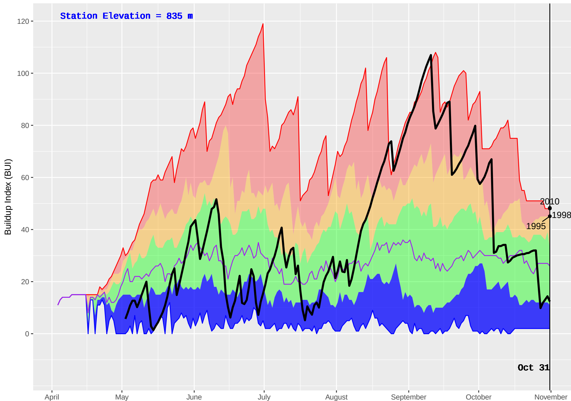
SILVER (120) : Historical (1986–2016) and Current (2017) Noon Buildup Index (BUI)
